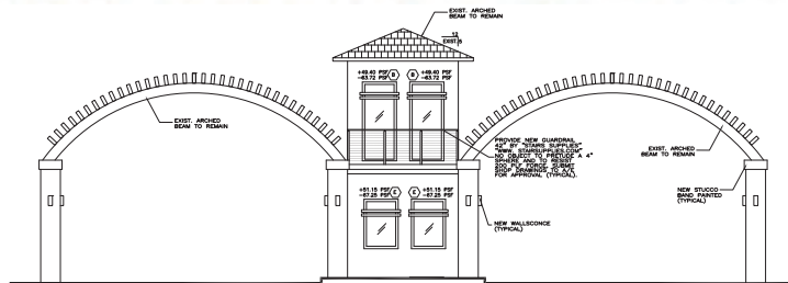
PROPOSED EAST ELEVATION SCALE: 1/4"=1'-0"
