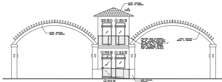
PROPOSED WEST ELEVATION SCALE: 1/4"=1'-0"
