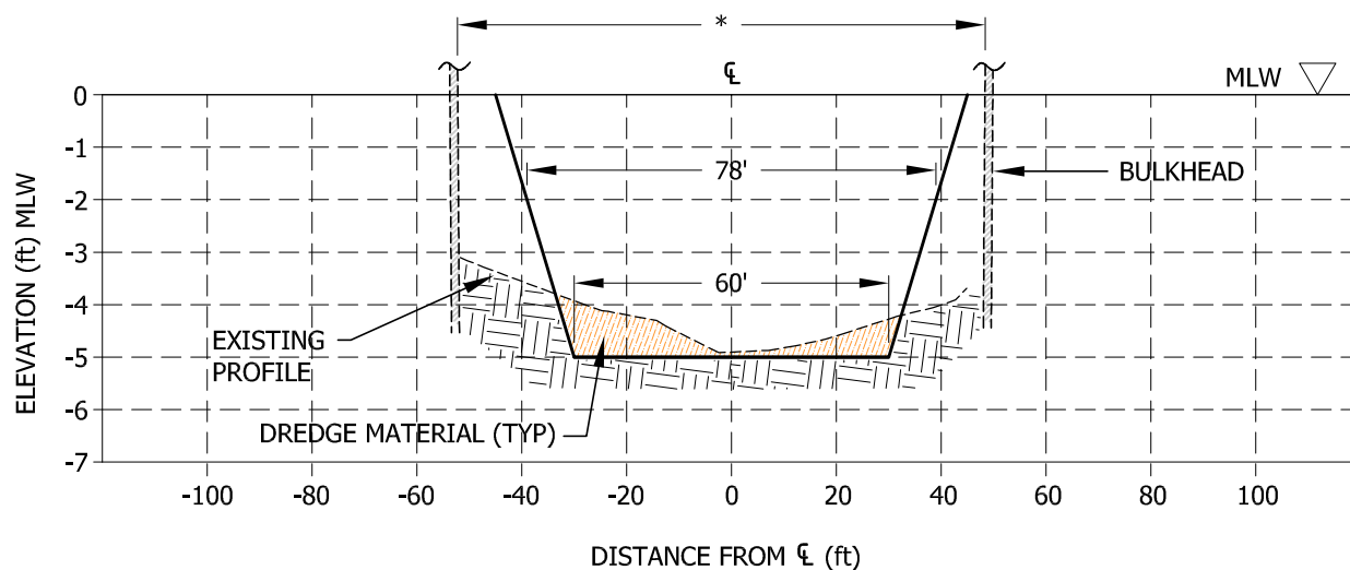
Section @ Sta. N 800'
