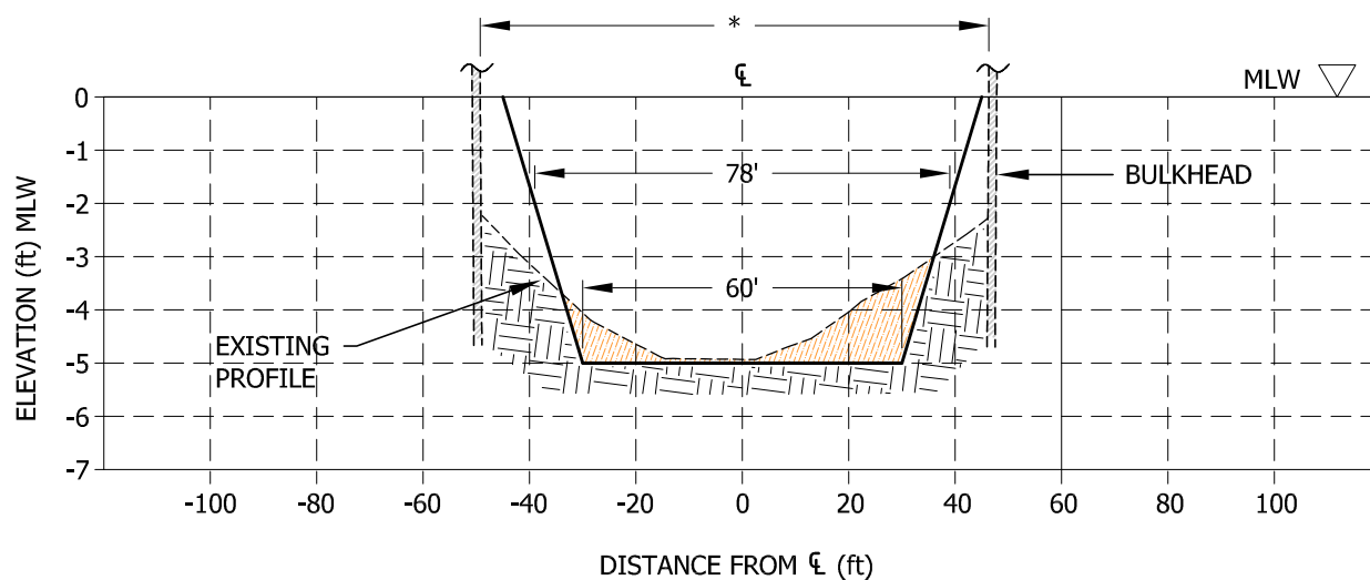
Section @ Sta. N 1200'
